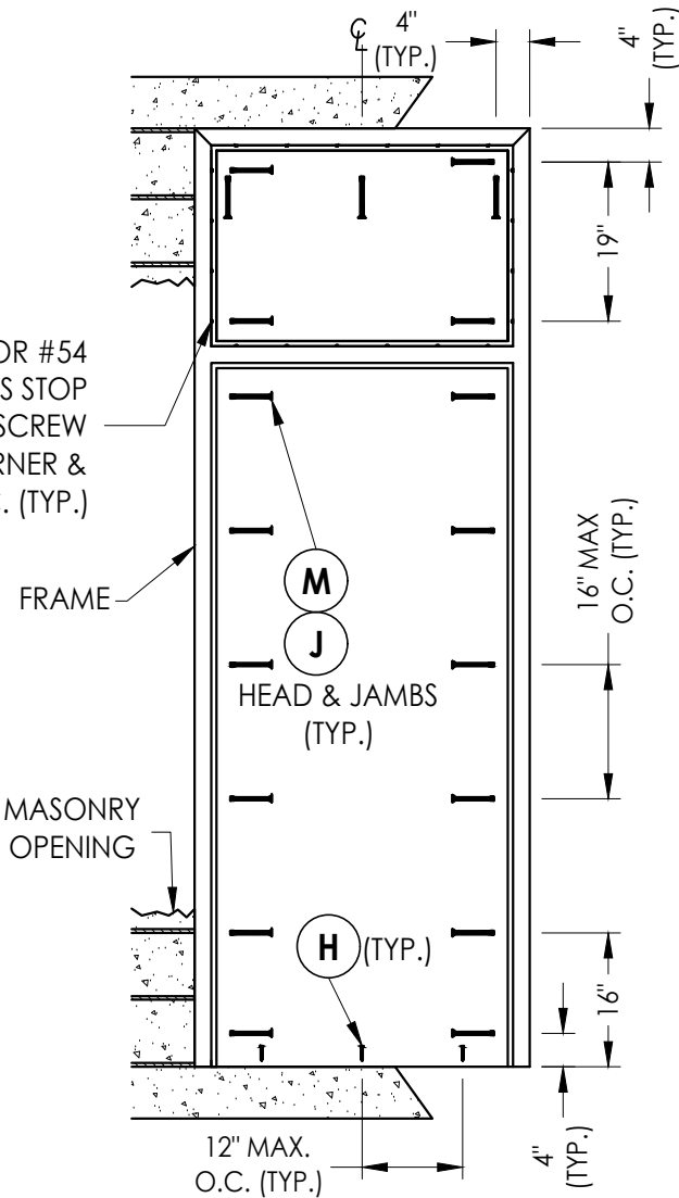
FRAME ANCHORING
